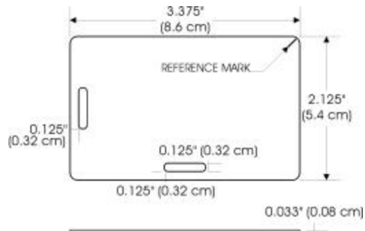
Prox-Line G Dimensions 3.375 x 2.125 x .033 inches (8.57 x 5.4 x .08 cm)
