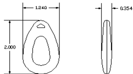
Prox-Line Dimensions 2.0 x 1.24 x .35 inches (5.08 x 3.15 x .89 cm)
