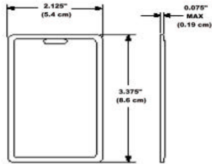
Prox-Line S Dimensions 3.375 x 2.125 x .075 inches (8.57 x 5.4 x .19 cm)
